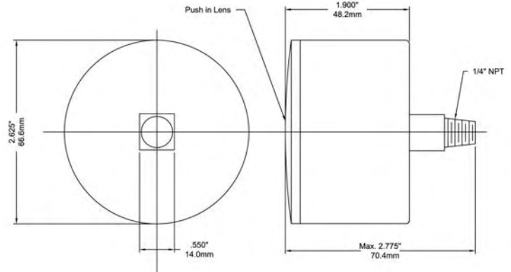
2.5" Back Connection Brass
