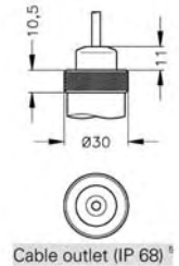
Cable outlet (IP 68) 5 5 Different cable types/lengths available
