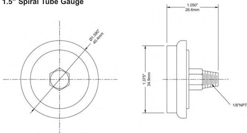
1.5" Spiral Tube Gauge
