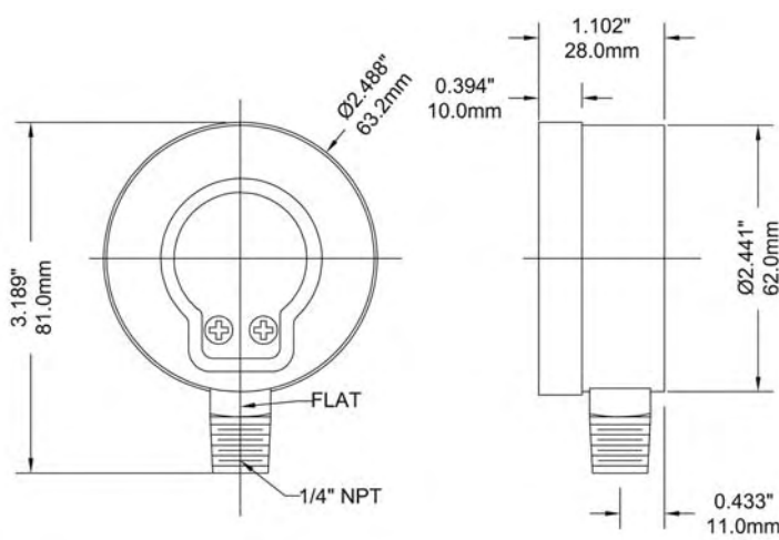
2.5" Bottom Connection
