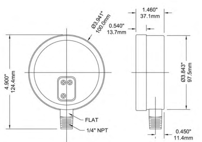
4" Bottom Connection
