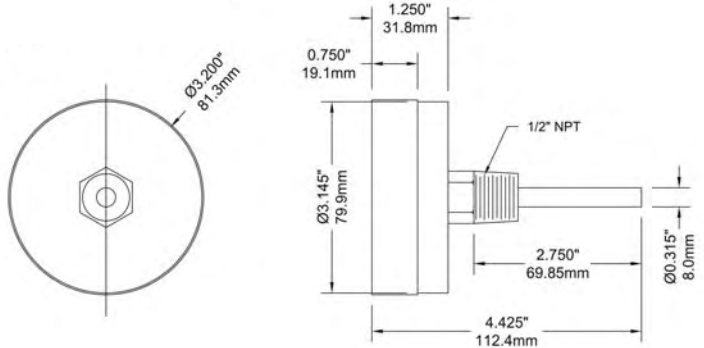
3" Back Connection
