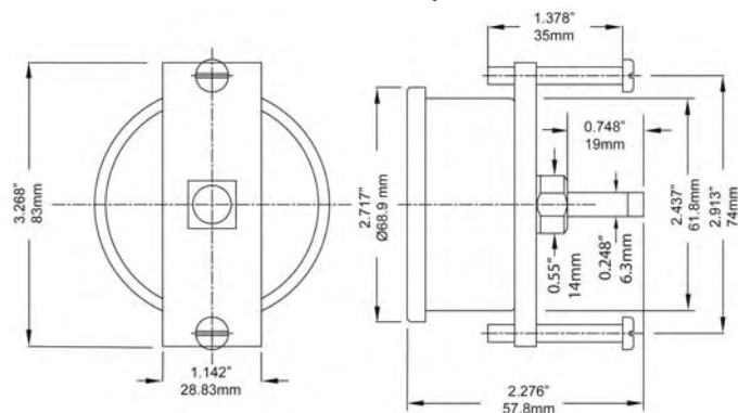
2.5" Back Connection with U-Clamp
