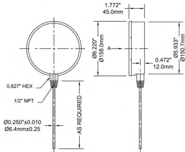
6" Bottom Connection
