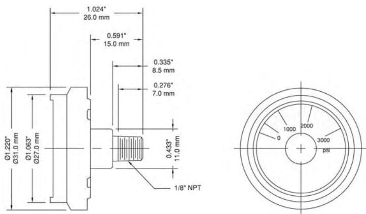
1 1/8" Spiral Tube Gauge
