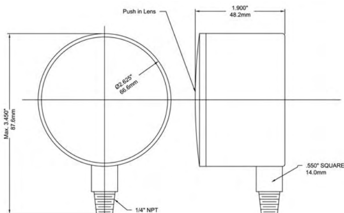
2.5" Bottom Connection Brass
