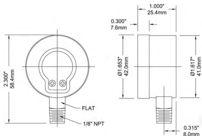
1.5" Bottom Connection
