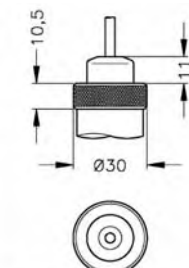
Cable outlet (IP 68) 7
