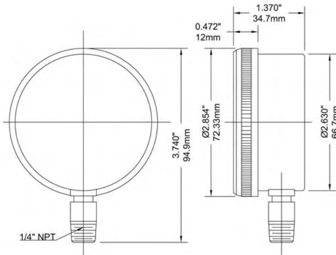
2.5" Bottom Connection
