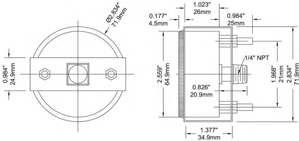
2.5" Back Connection, U-Clamp
