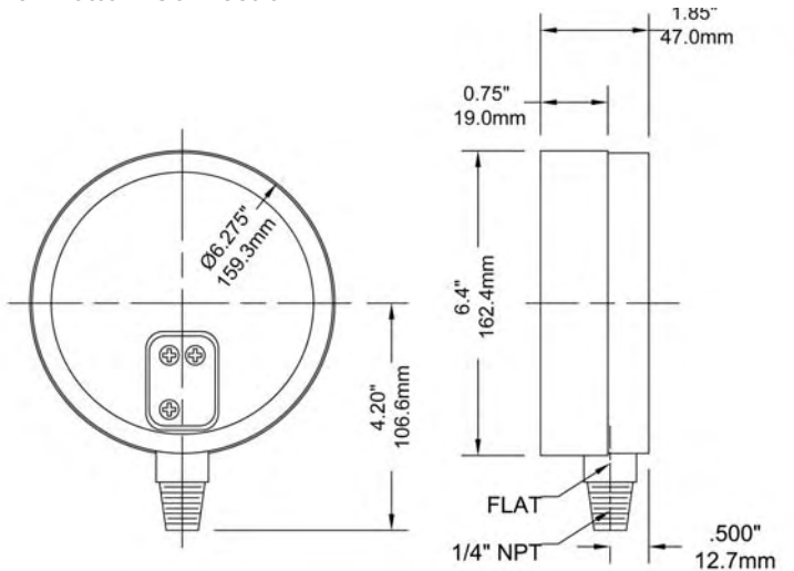
6" Bottom Connection
