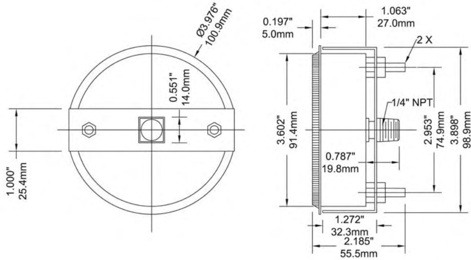
3.5" Back Connection, U-Clamp
