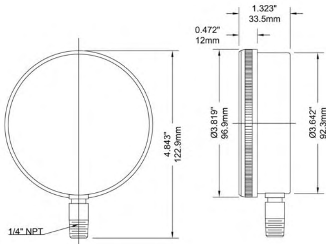
3.5" Bottom Connection
